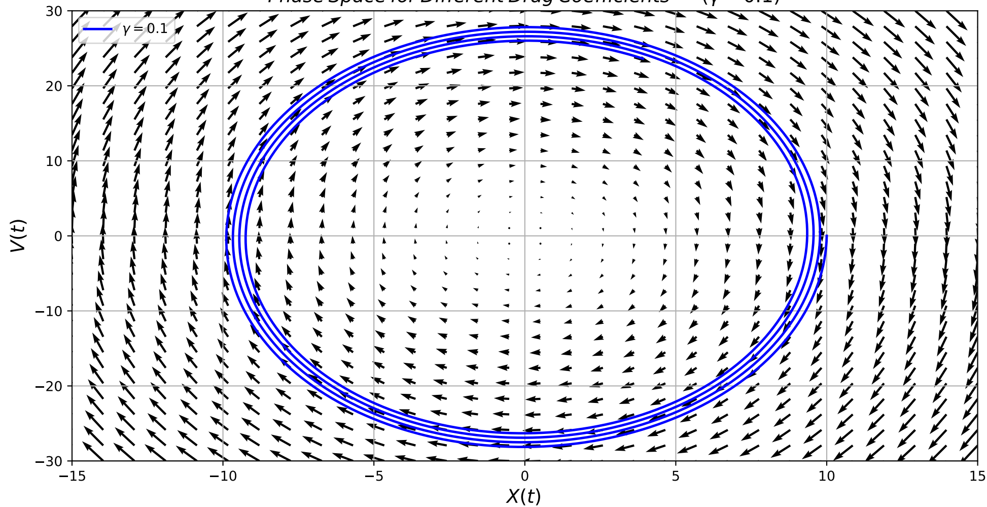
Phase Space for Different Drag Coefficients – ( \gamma = 0.1 )
